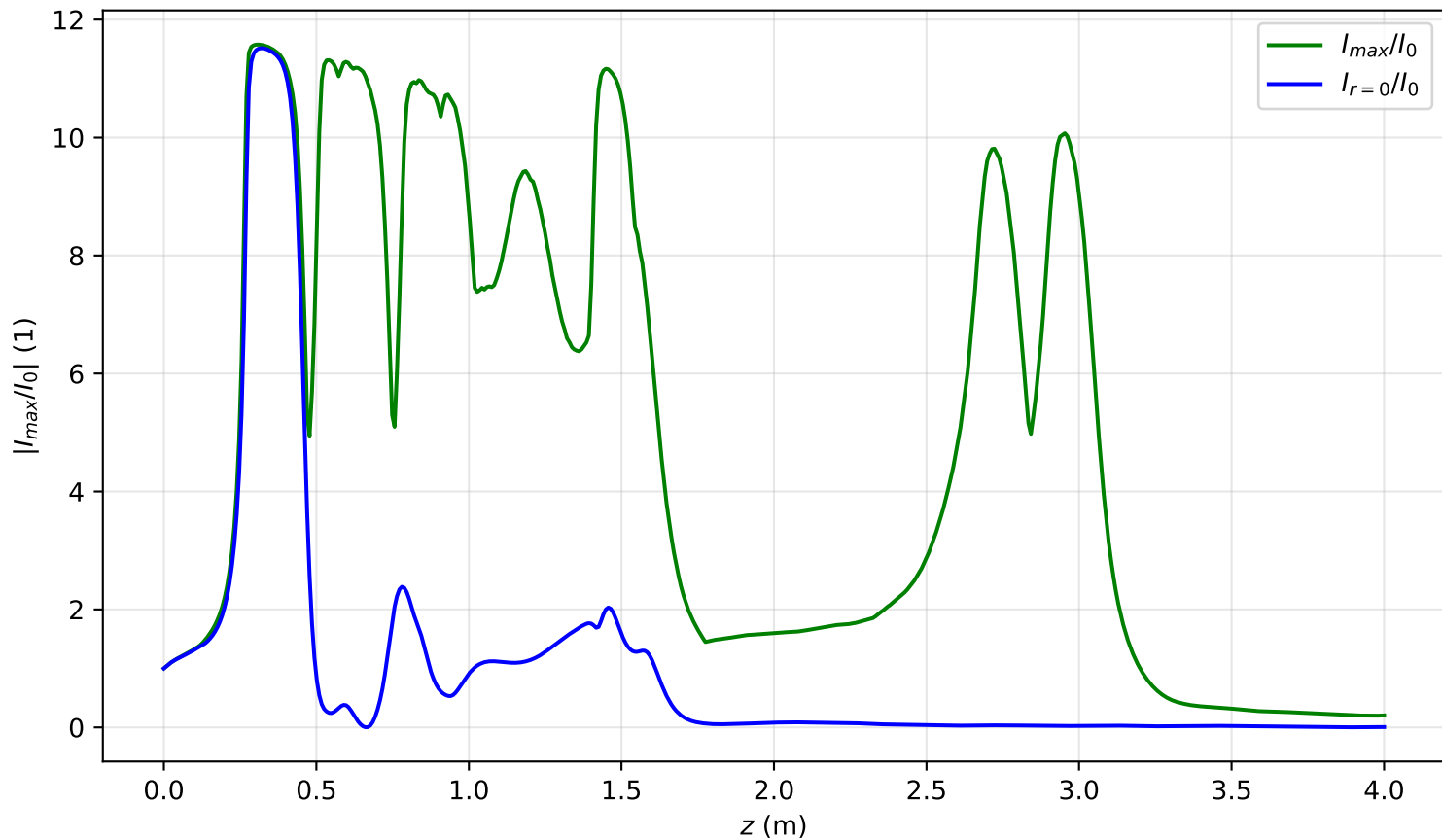
I_{max}(x=0, y=0, z)/I_0 , Pin=9.6Pcr, noisy input, artificial time
